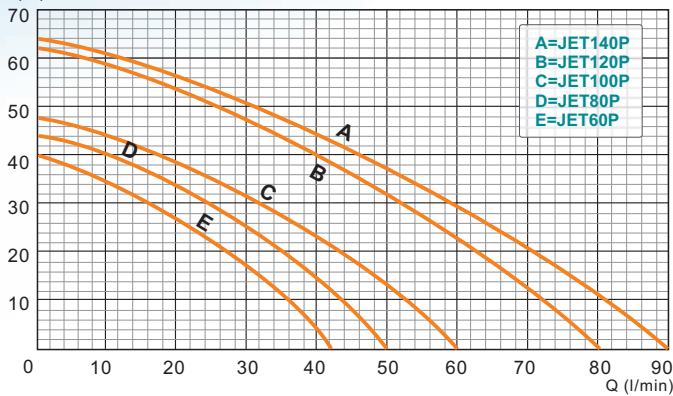
H (m) PERFORMANCE CHART AT n=2850 min -1
